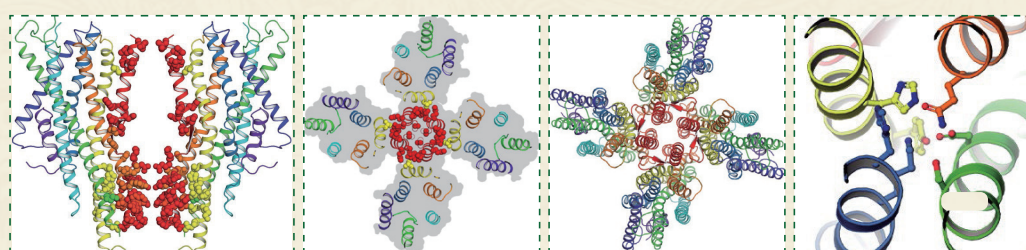
Architecture of the Orco homotetramer
